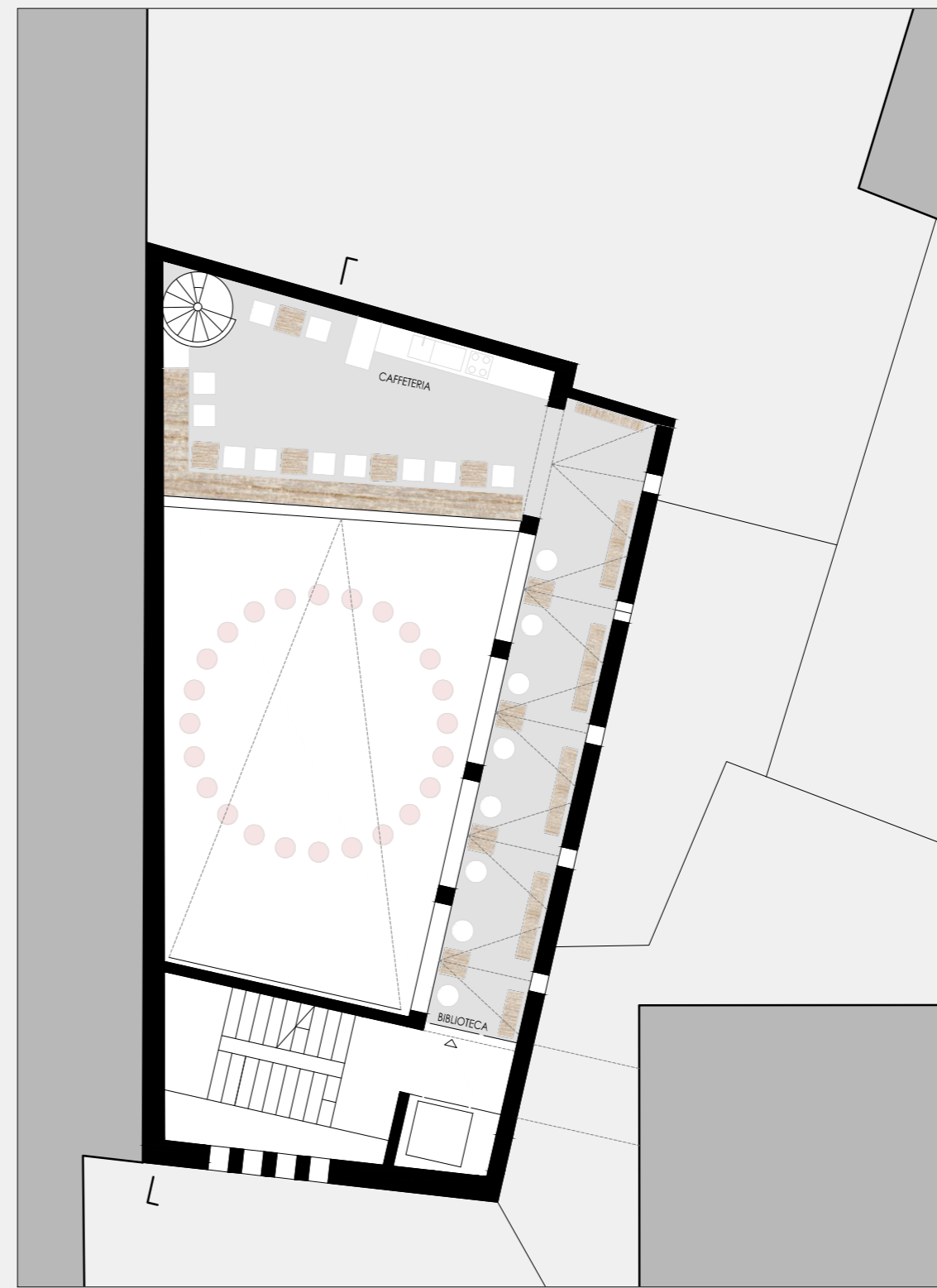
⊗ 1.OBERGESCHOSS | PIANO PRIMO
